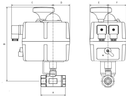
FIG 241-EA - with Electric Actuator
