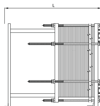
BOSS Model BM10B Plate Heat Exchanger
