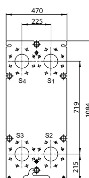
BOSS Model BM10M Plate Heat Exchanger
