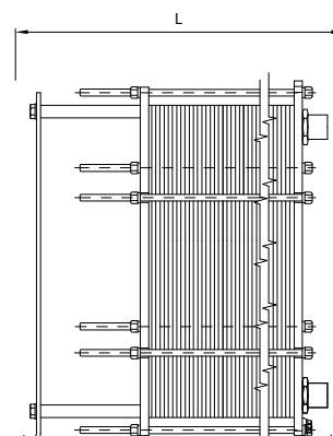
BOSS Model BM6 Plate Heat Exchanger
