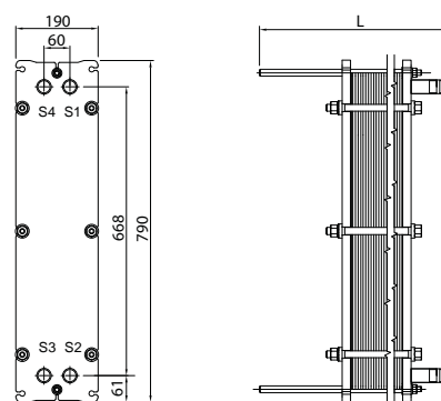
BOSS Model BTL3 Plate Heat Exchanger
