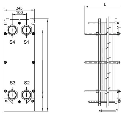
BOSS Model BT5B Plate Heat Exchanger
