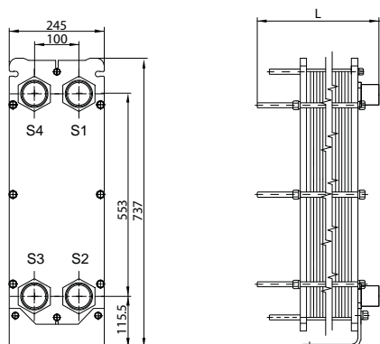
BOSS Model BT5M Plate Heat Exchanger
