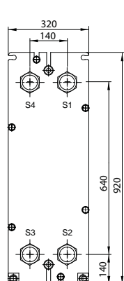
BOSS Model BM6M Plate Heat Exchanger
