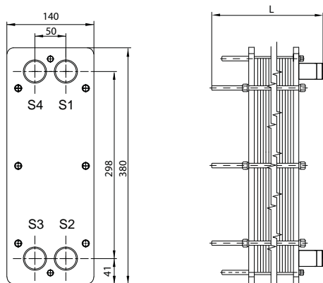
BOSS Model BT2 Plate Heat Exchanger
