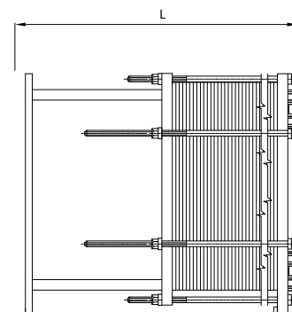
BOSS Model BM10M Plate Heat Exchanger
