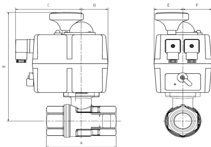
FIG 250-EA - with Electric Actuator
